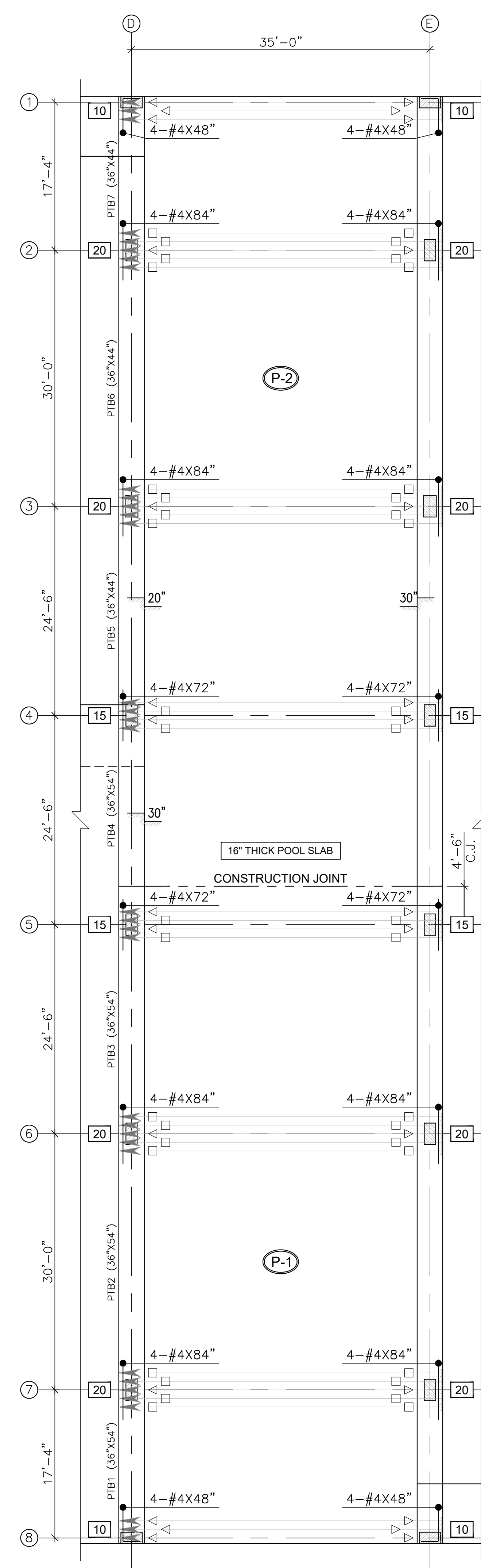
B PARTIAL PLAN POOL SLAB
