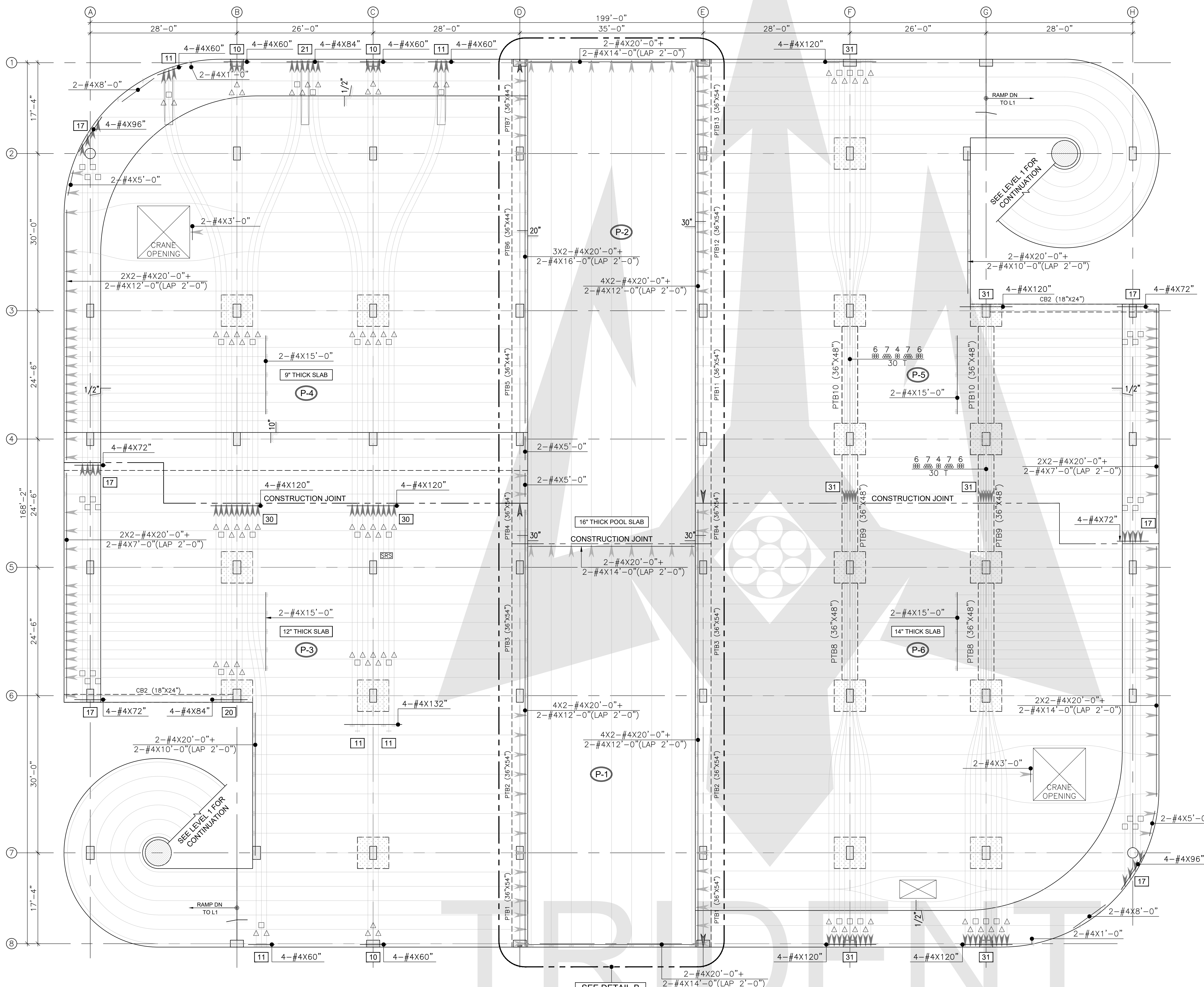
PT-REBAR CALCULATION LAYOUT LEVEL 2
